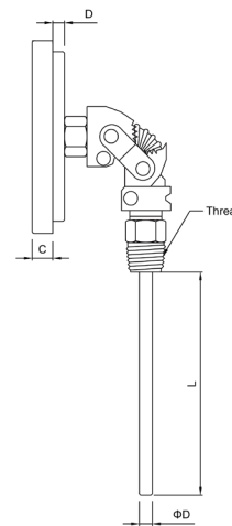
DA Adjustable angle mount
