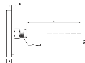
DT Back mount
